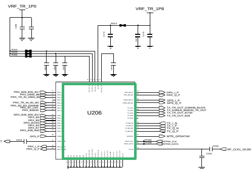
RF Transceiver
