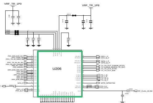
RF Transceiver
